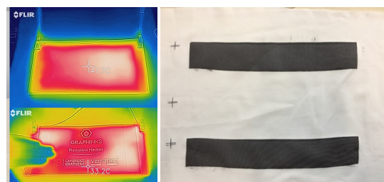
Graphink 2/CMC screen printed patterns on paper (top), Meyer bar coatings for electrothermal heater applications (left), screen printed conductive circuits on textiles (right).
